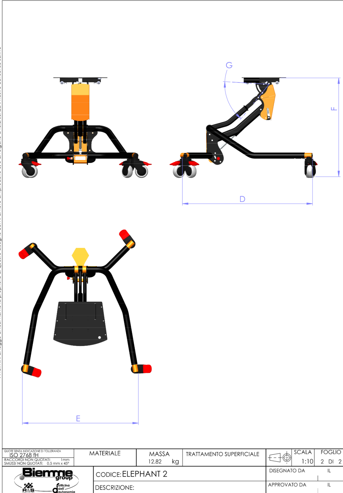
Fig. 1 Technical drawing of the device
